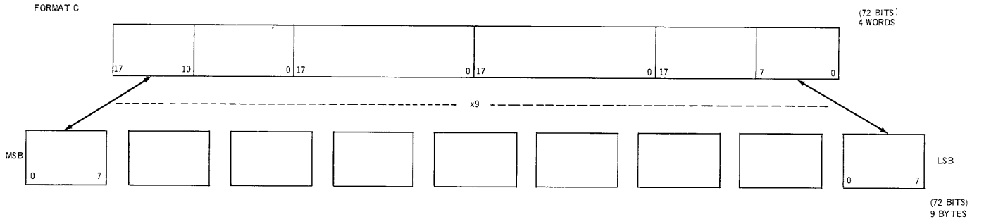
Figure 6-1. ICCU Data Formats
